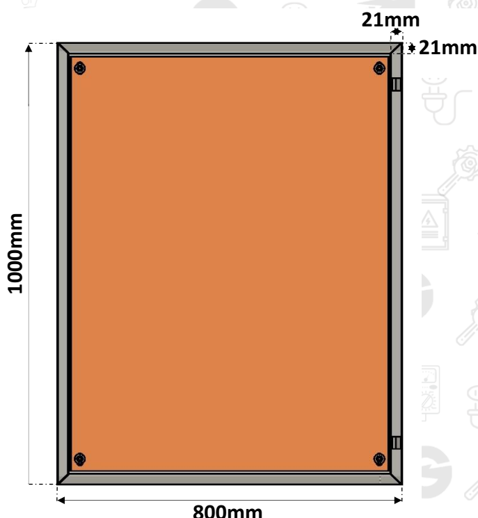
PORTA CHAPA 20# 0,90mm
